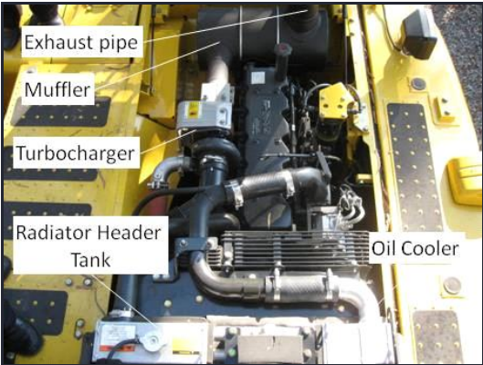
Engine components
