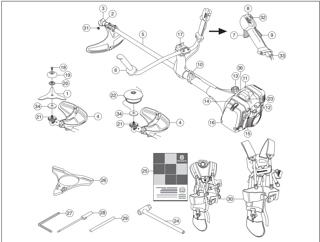
What is what on the brush cutter? (545 RX, 545 RXT)
